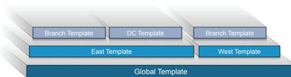
Figure 3: Template Stacking
